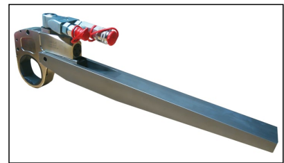
Support extension
